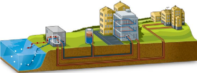
Figure 3: Layout of district cooling using free cooling with sea water
