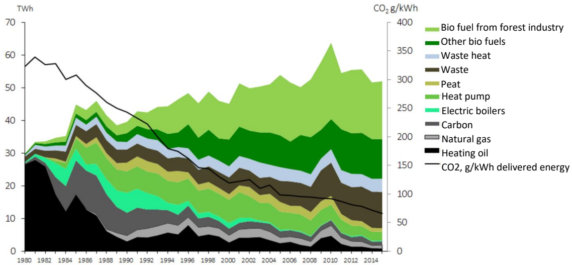
Figure 7: Fuel use for district heating in Sweden, 1980-2015
