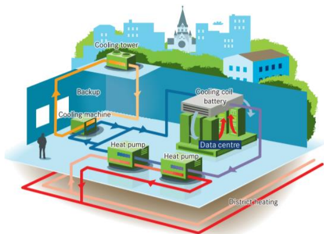
Figure 5: Open District Heating© implemented as a cooling solution in a data center. The existing cooling system is used for redundancy.
